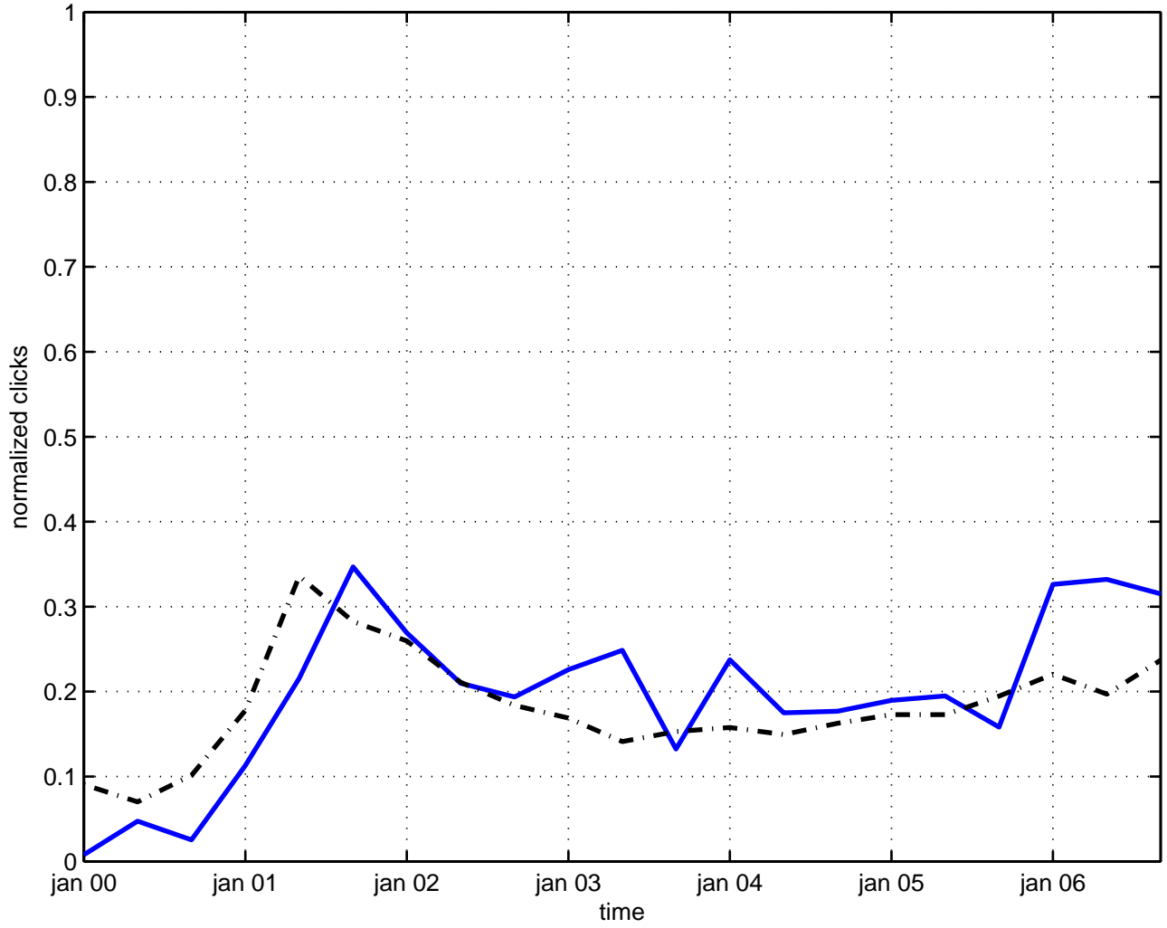
noncommutative space-time
