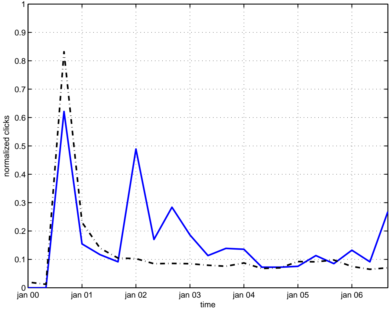
noncommutative renormalization
