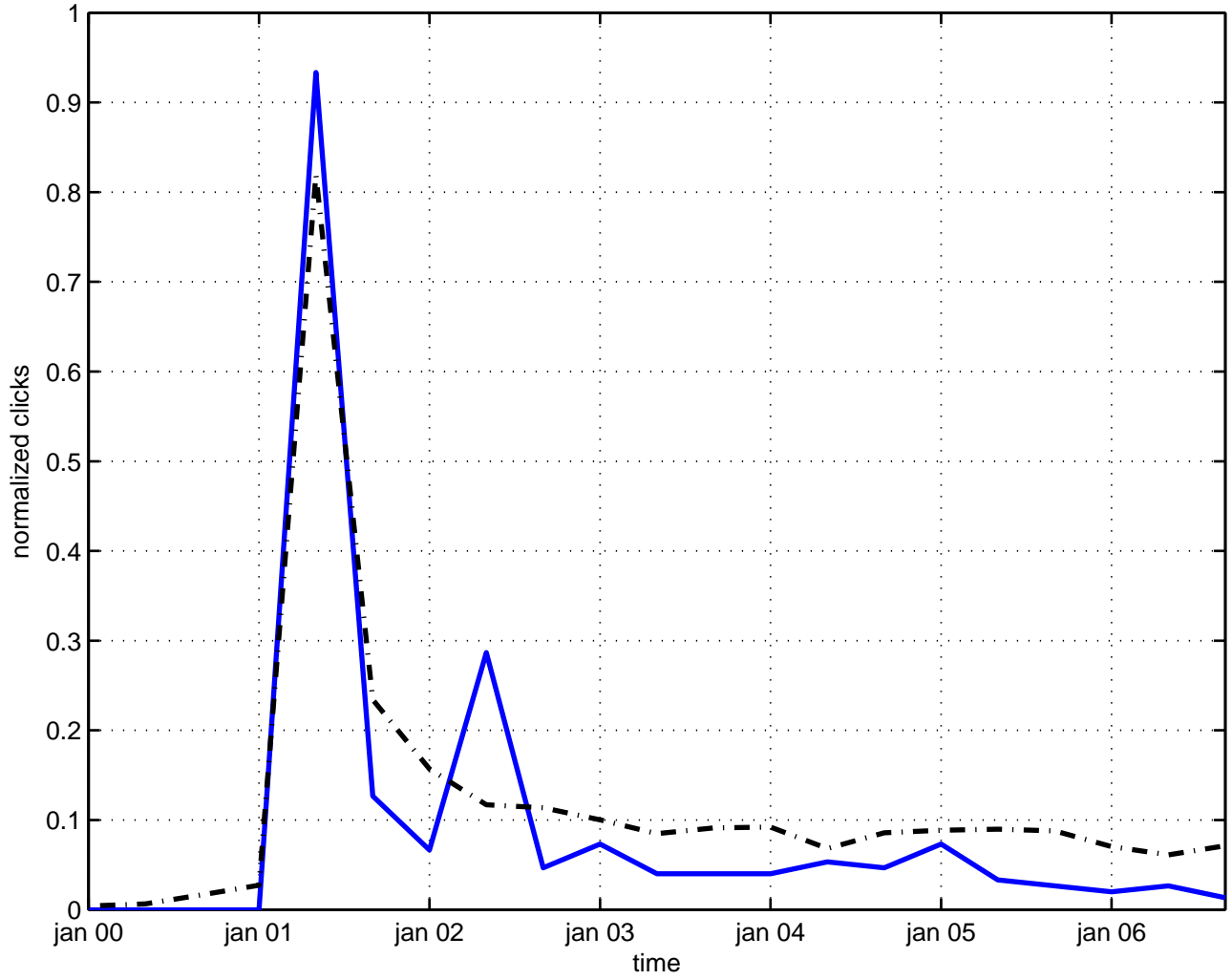
noncommutative quantization
