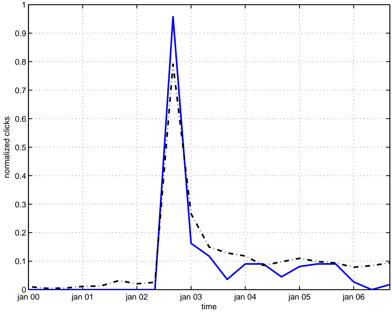
noncommutative particle
