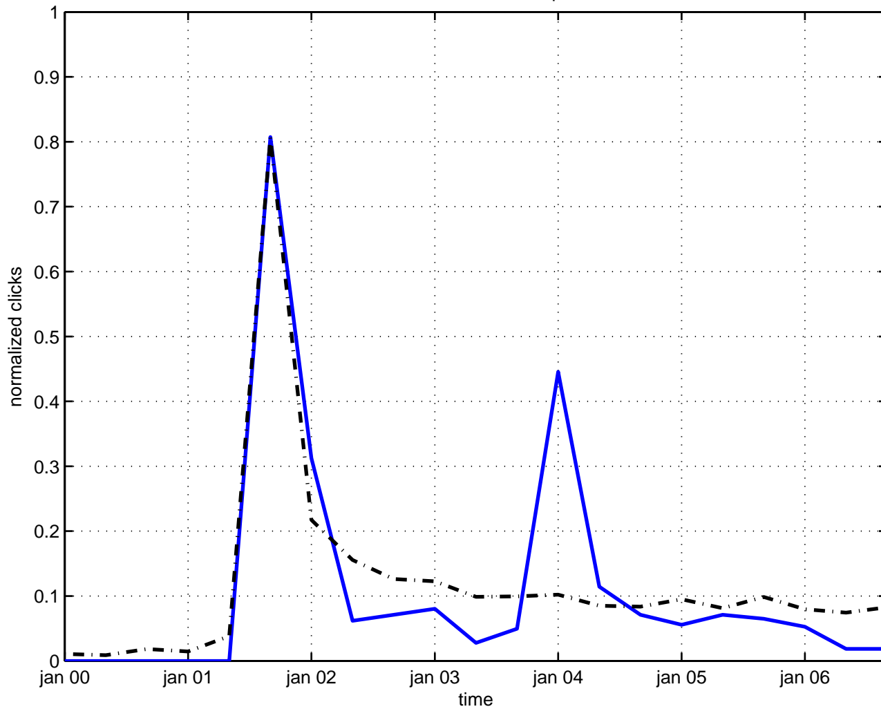
noncommutative monopole
