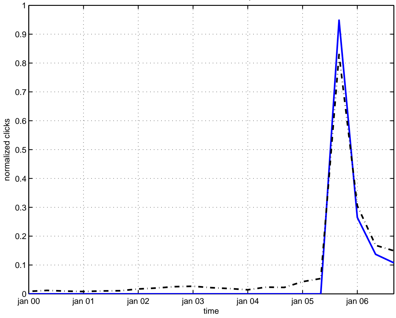
noncommutative moduli space
