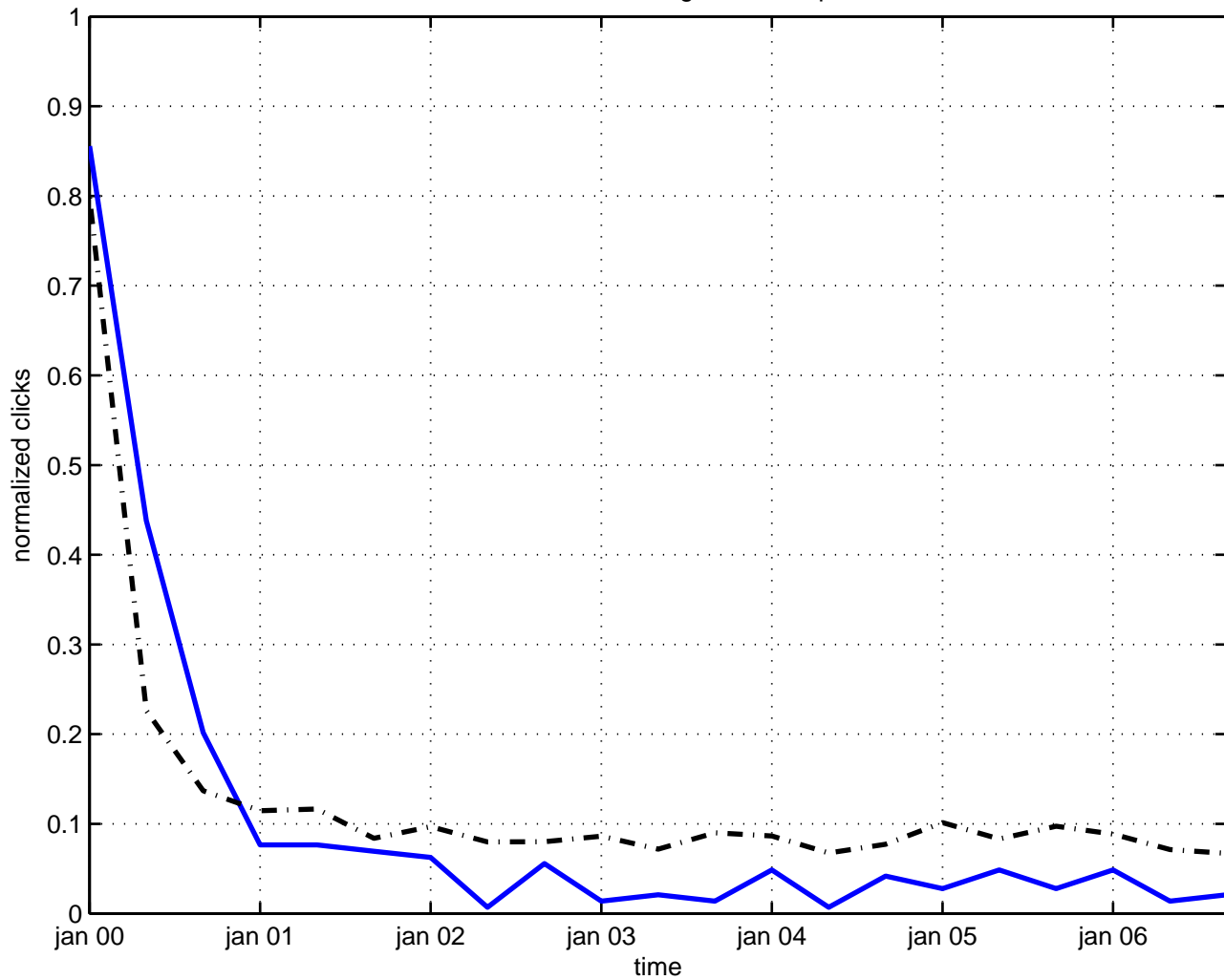
noncommutative magnetic monopole
