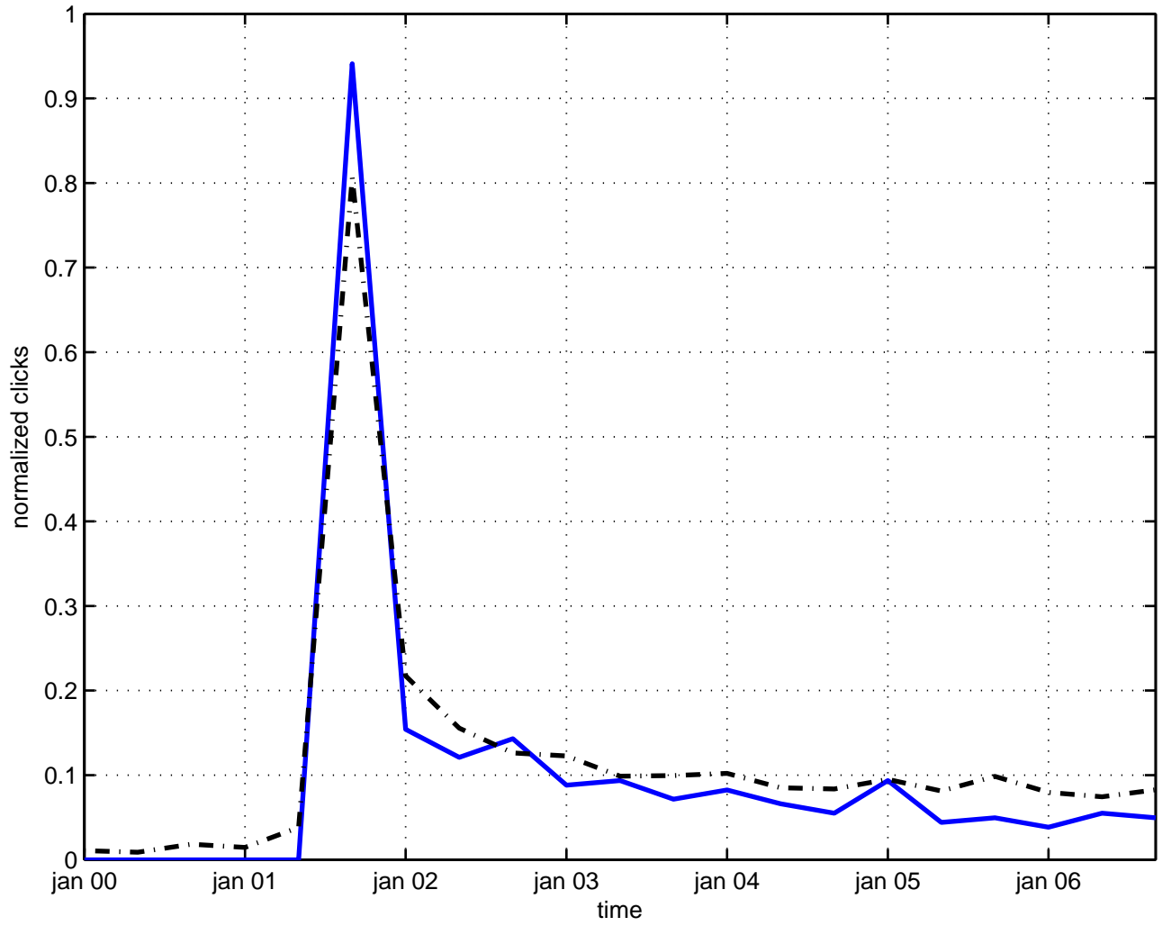
noncommutative landau-ginzburg model
