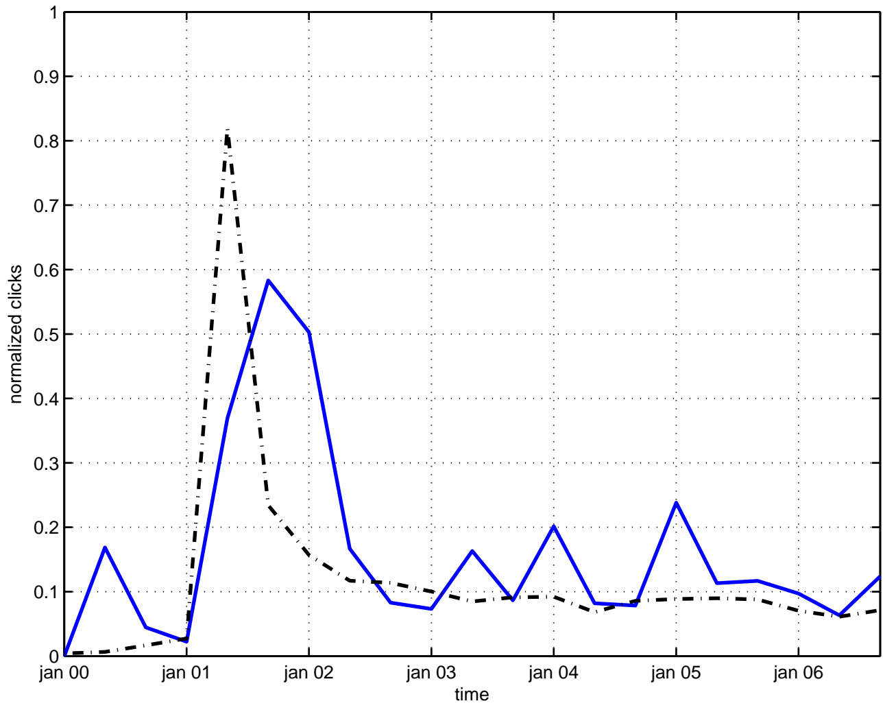
noncommutative instanton
