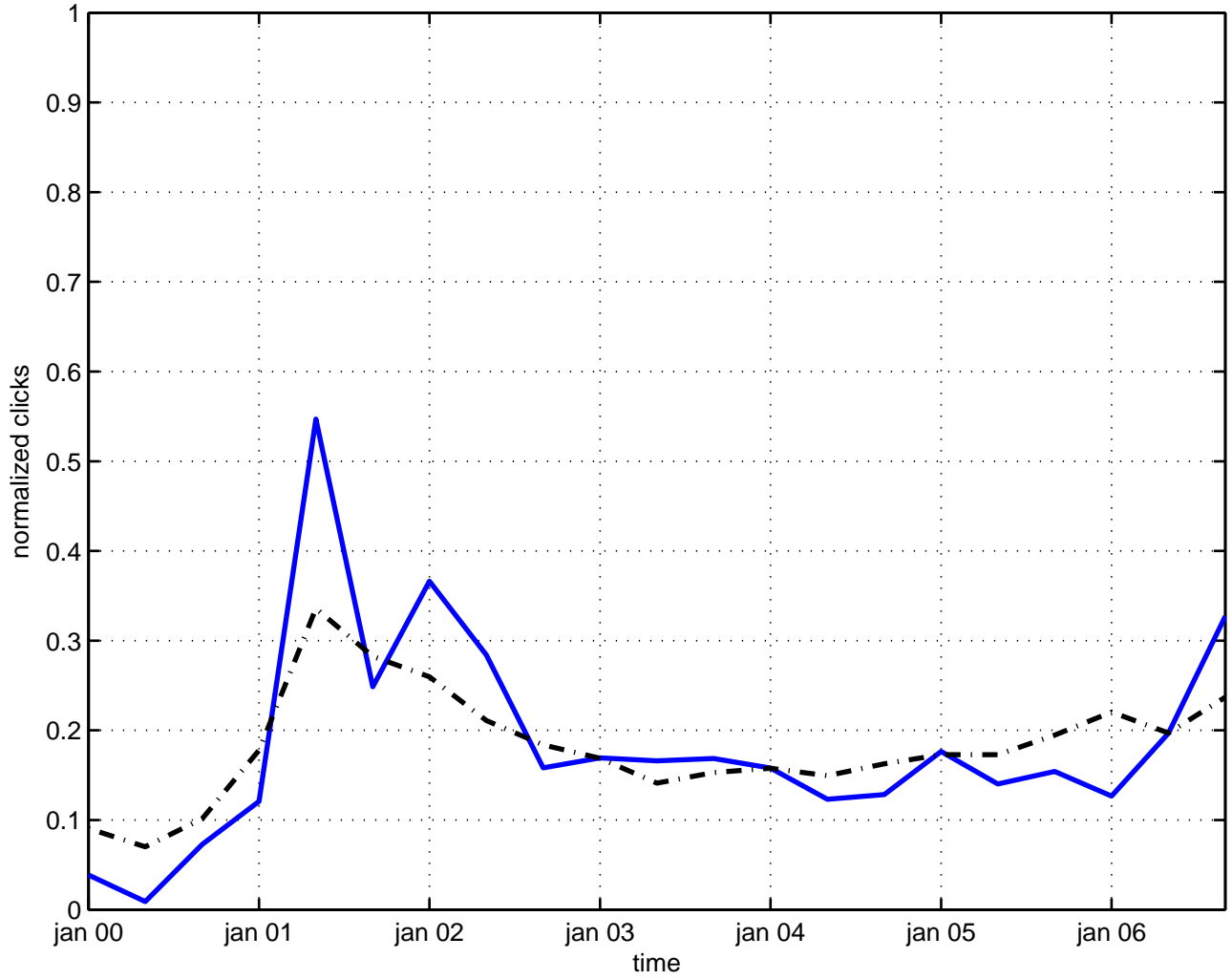
noncommutative geometry
