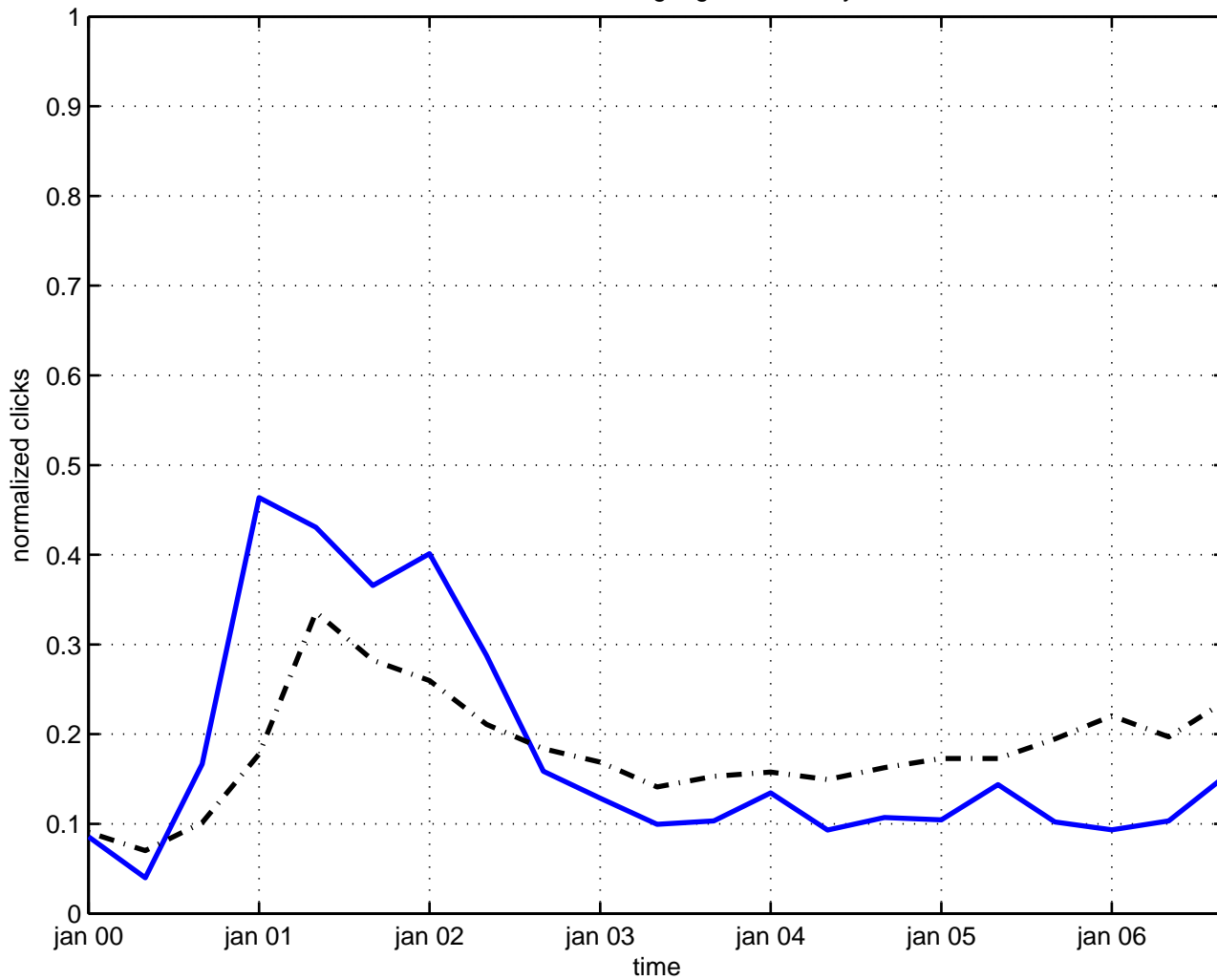
noncommutative gauge field theory
