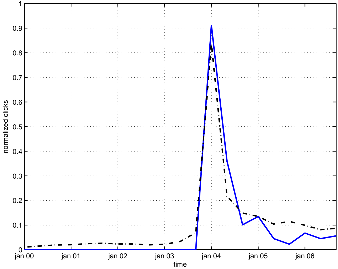
noncommutative four-fermion interaction
