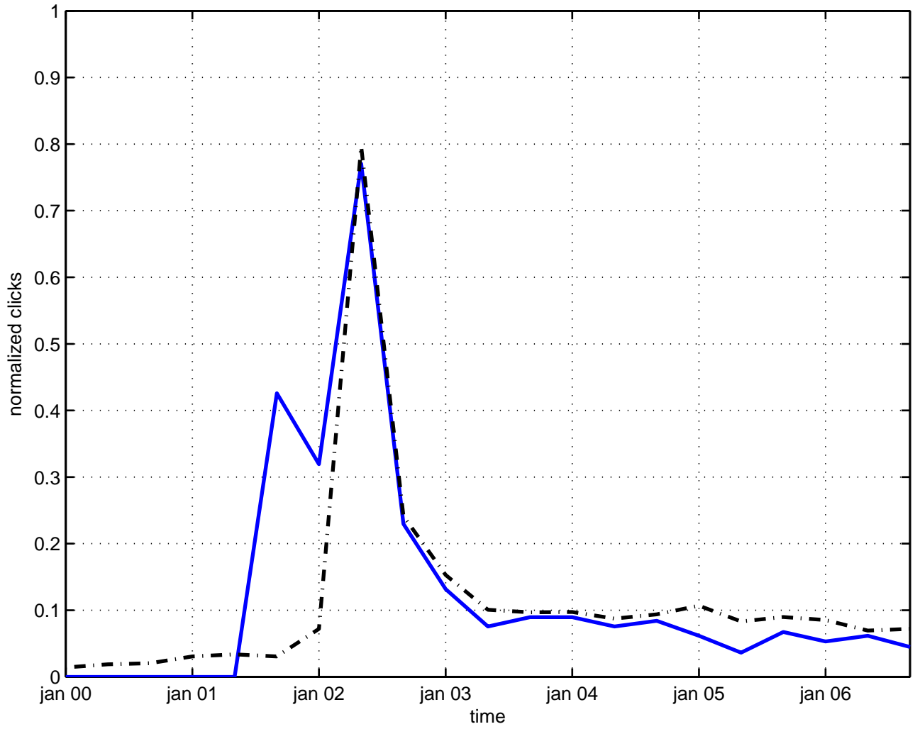
noncommutative dipole
