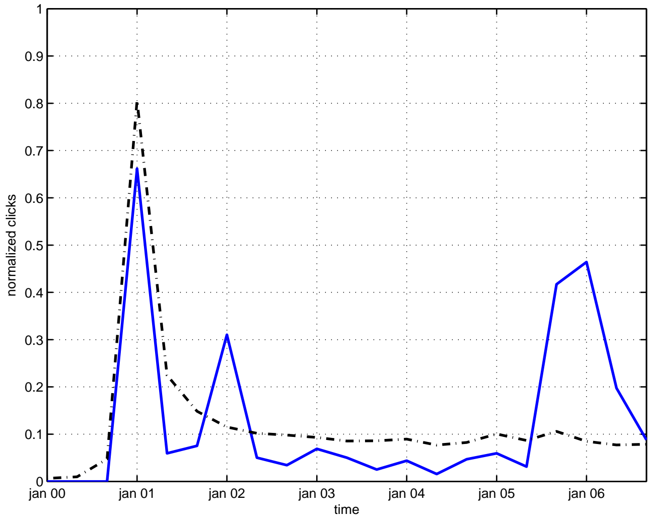
noncommutative deformation
