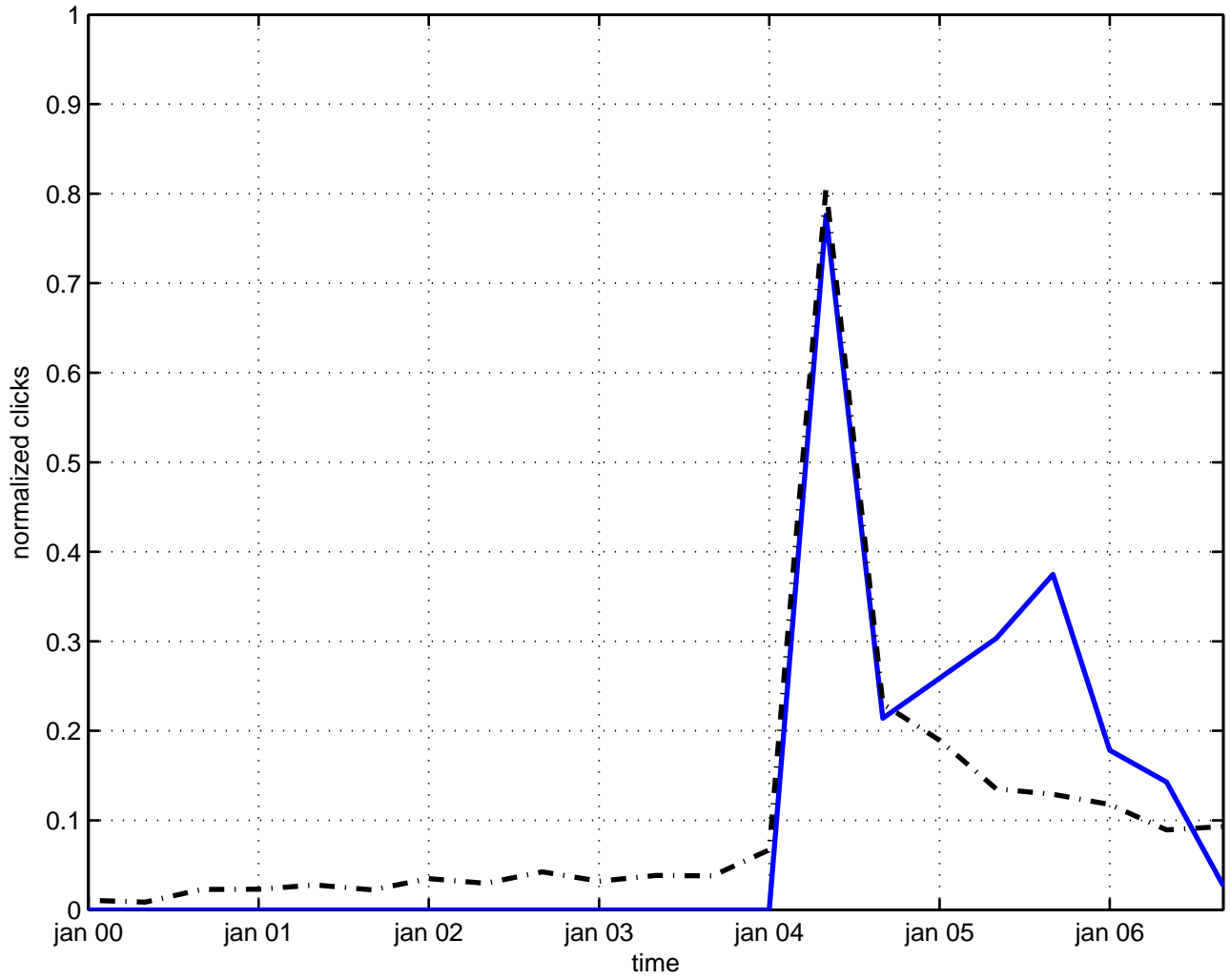
noncommutative correction
