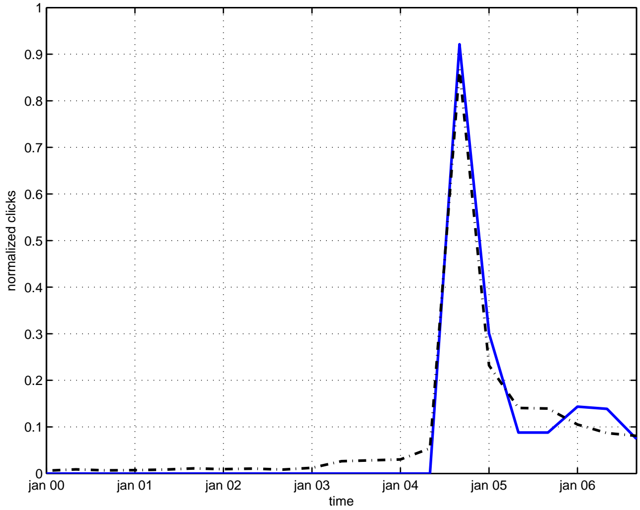
noncommutative central charge
