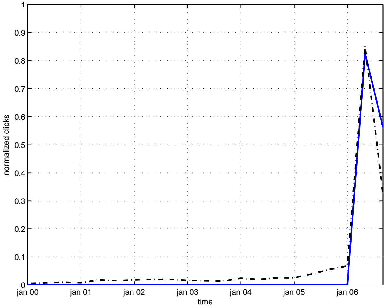
noncommutative black hole
