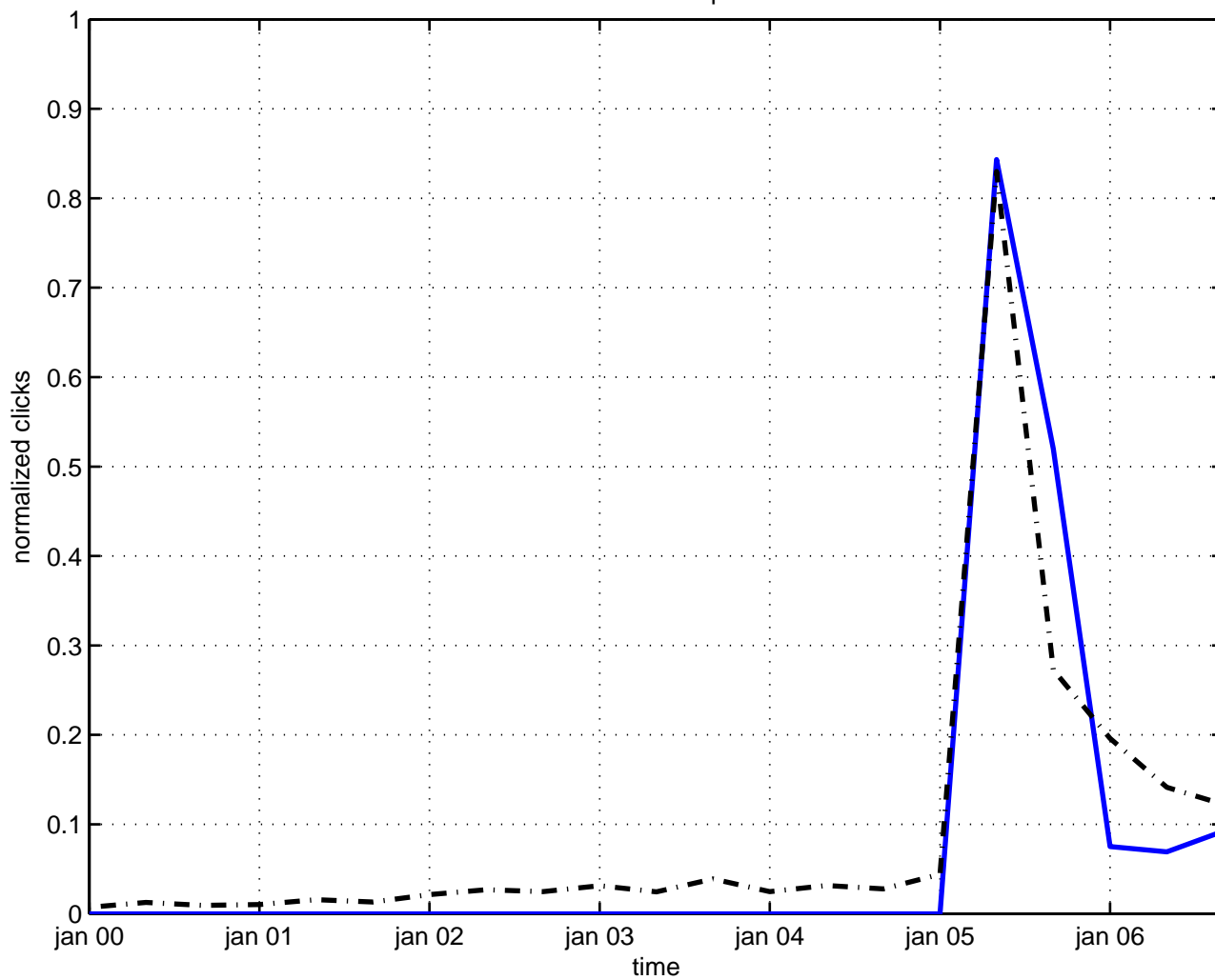
nonassociative operator
