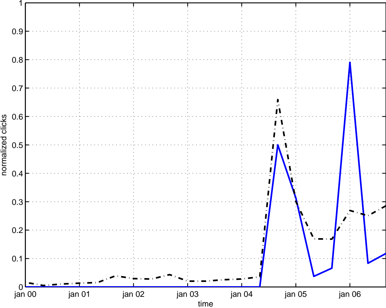
nonassociative gauge field theory
