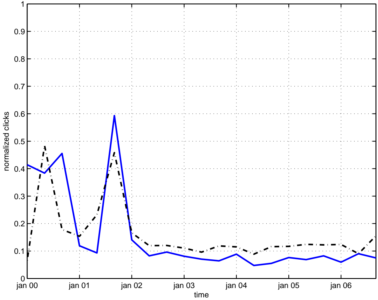
nonabelian orbifold
