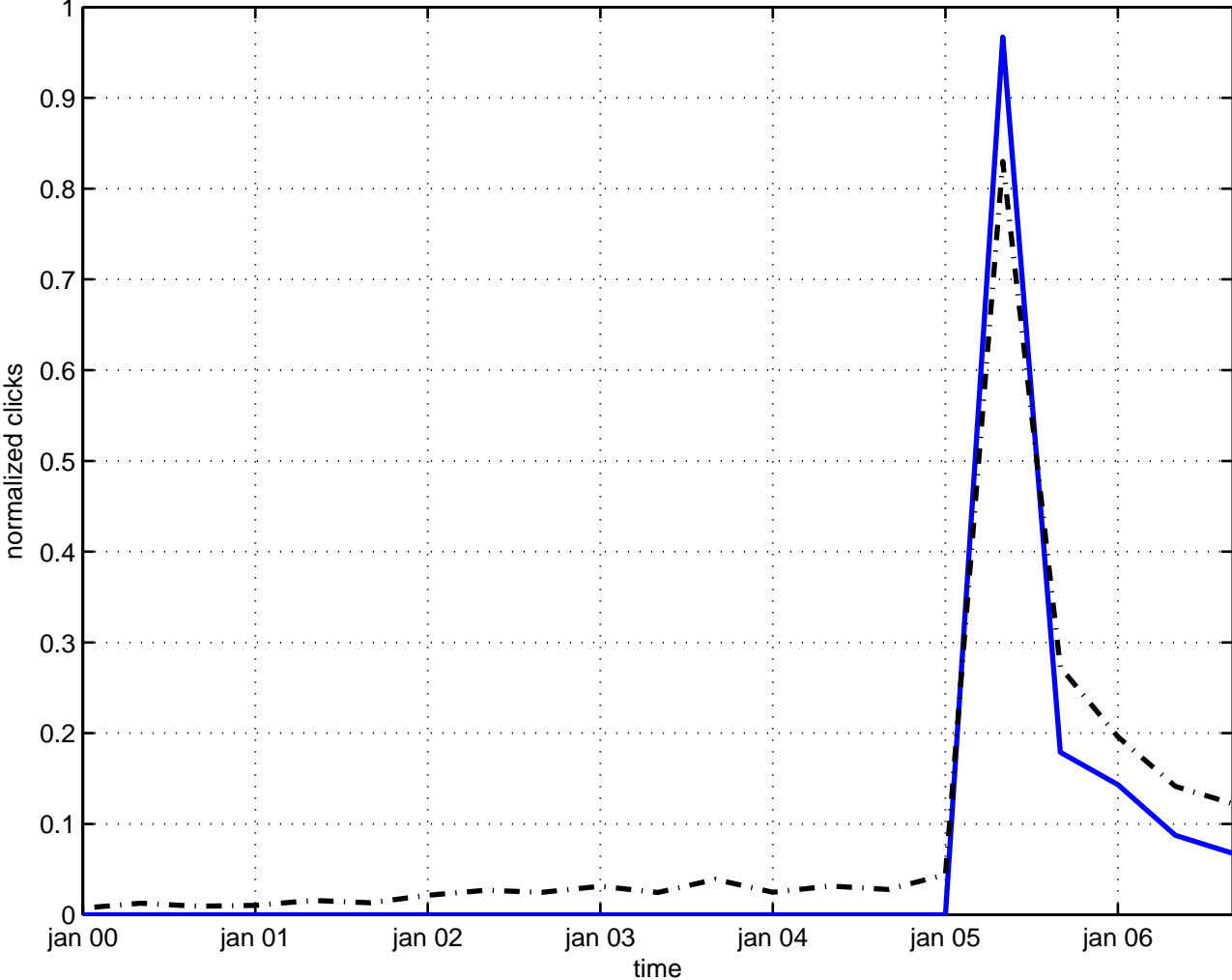
nonabelian network
