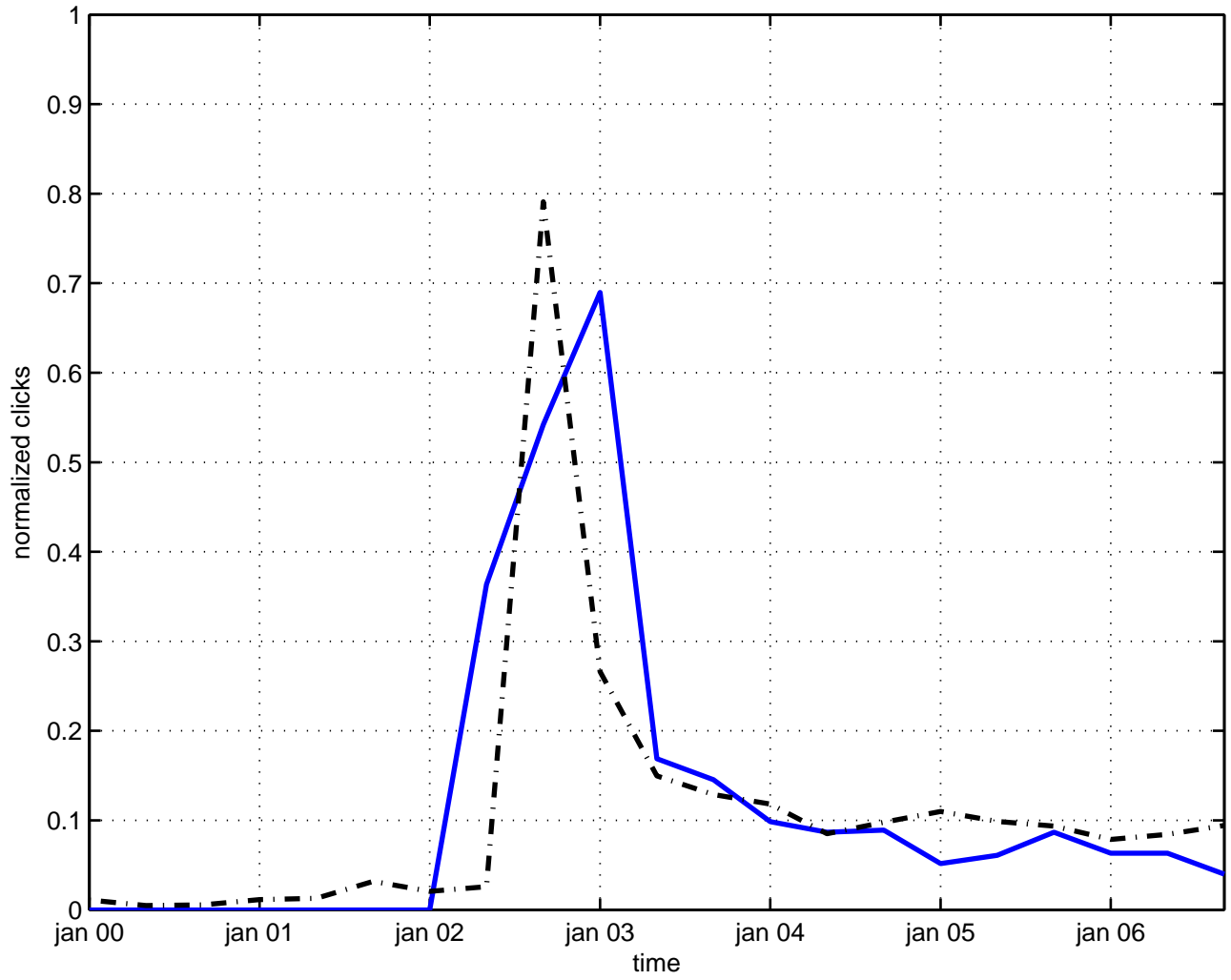
nonabelian magnetic monopole
