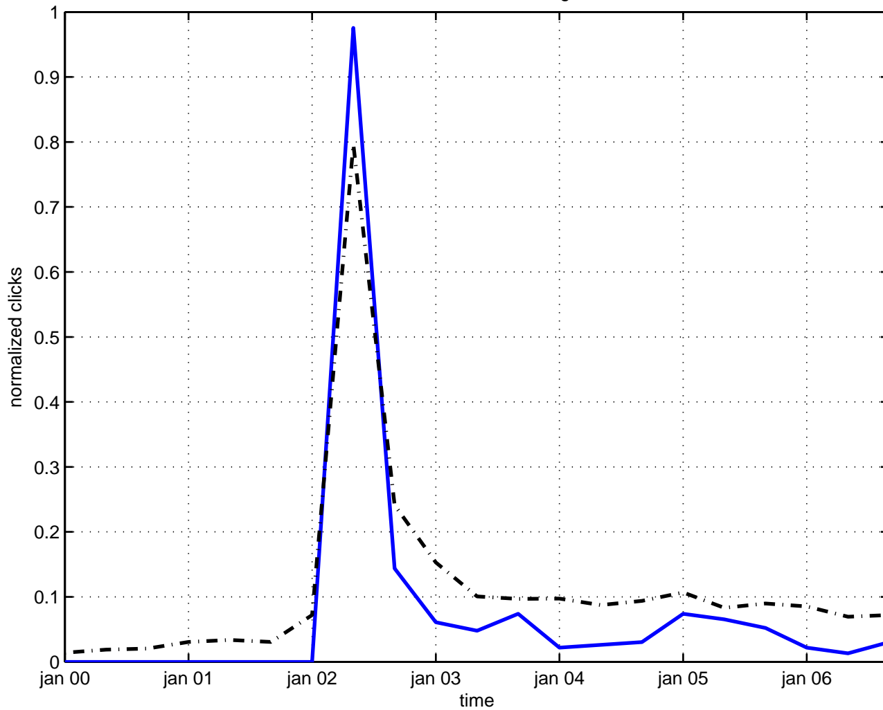
nonabelian embedding
