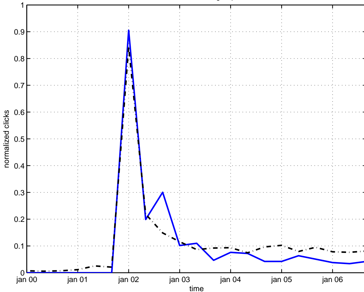
nonabelian braid group
