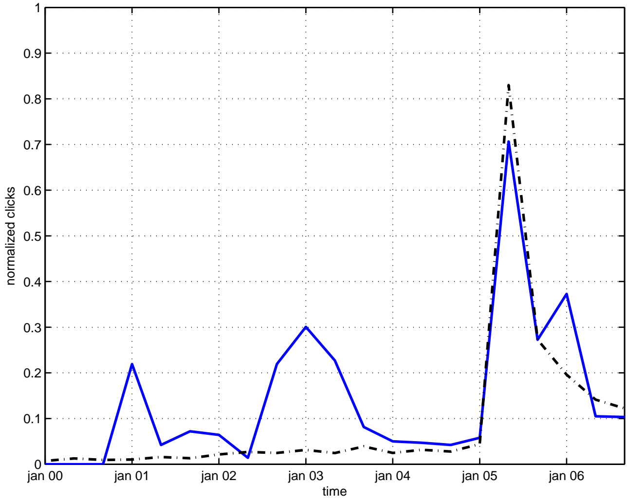
noether charge
