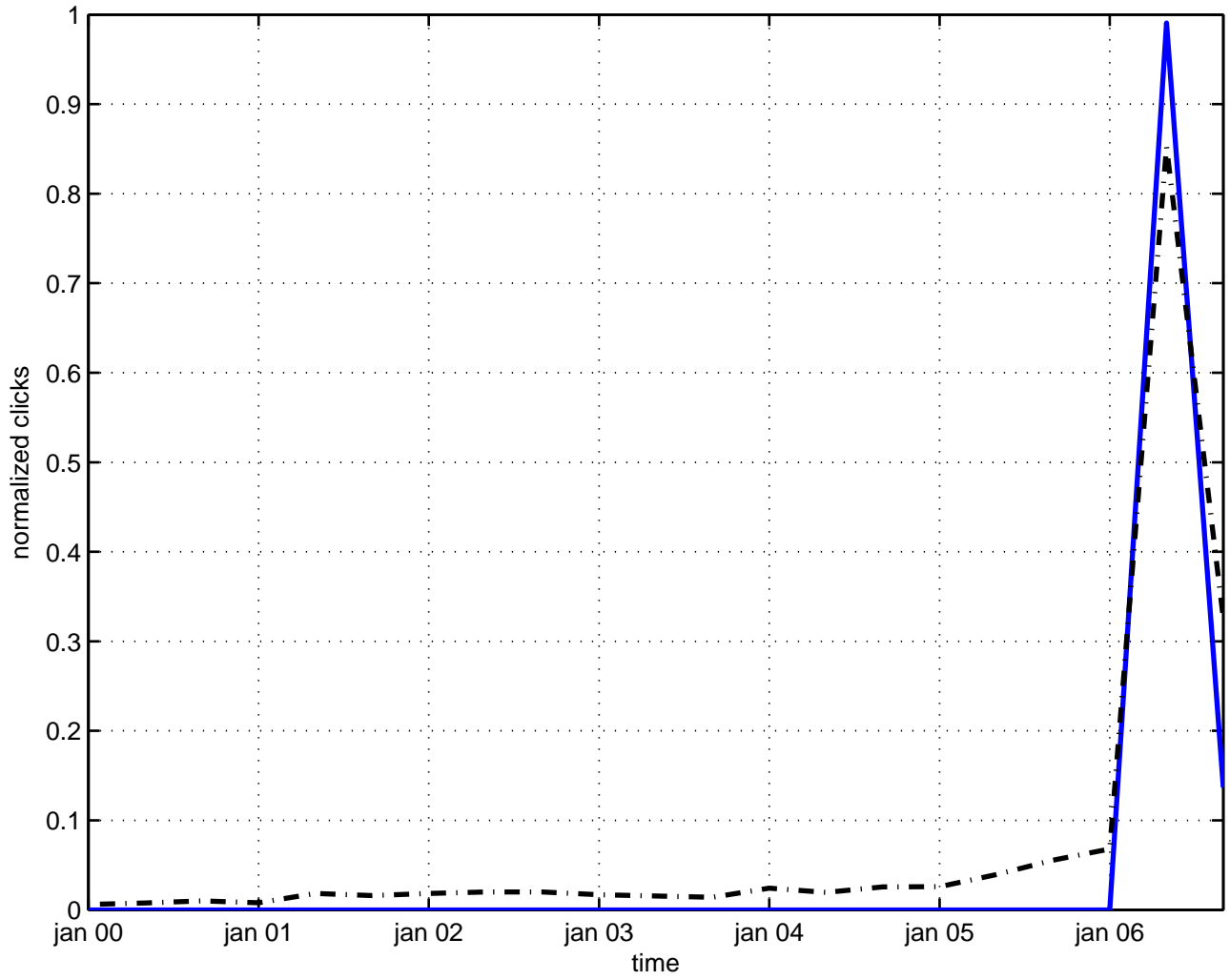
network superstring
