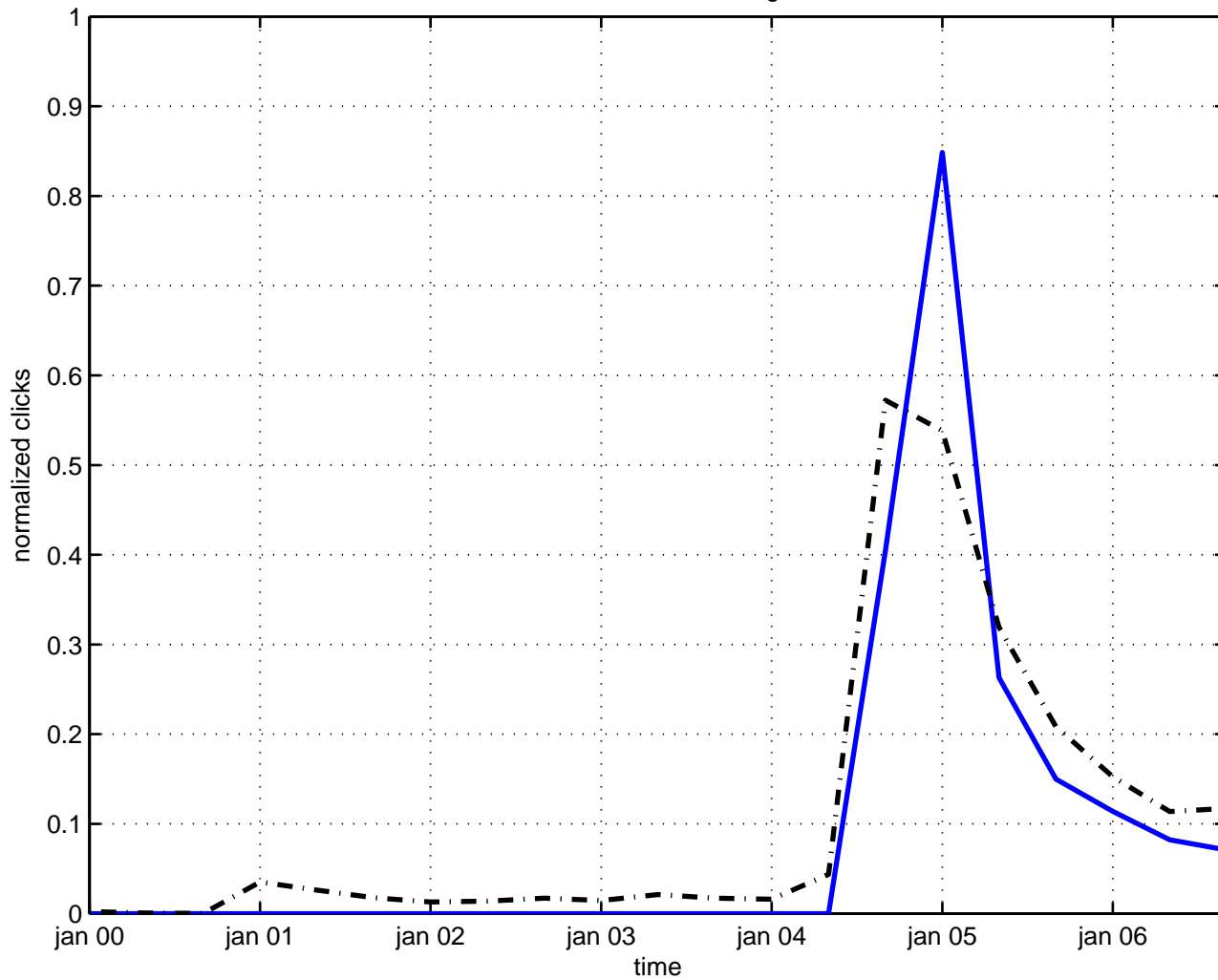
network cosmic string
