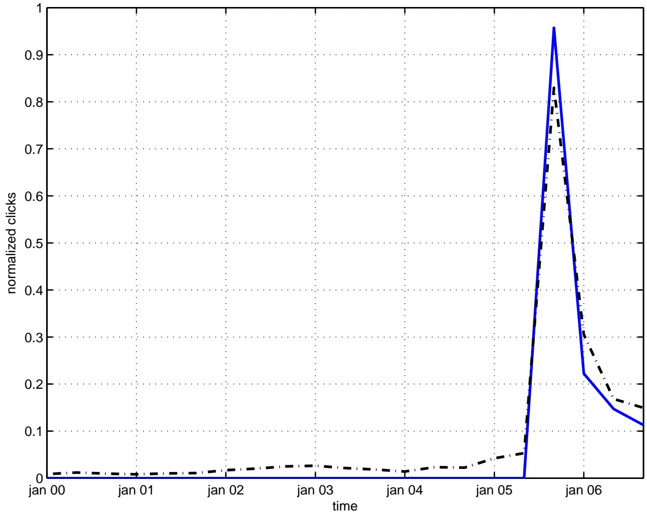
navier-stokes equation
