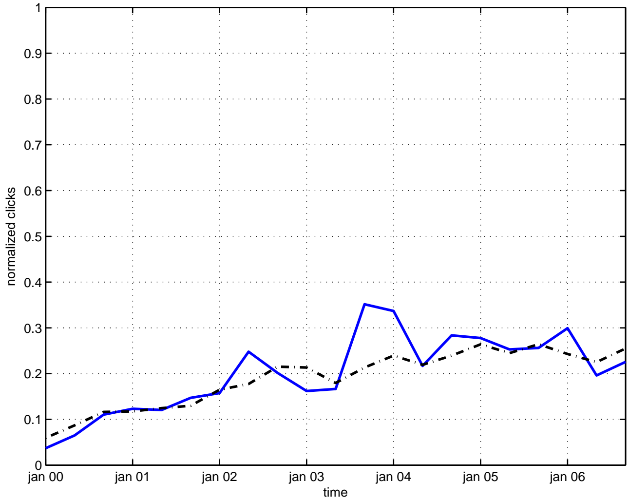
n-point function
