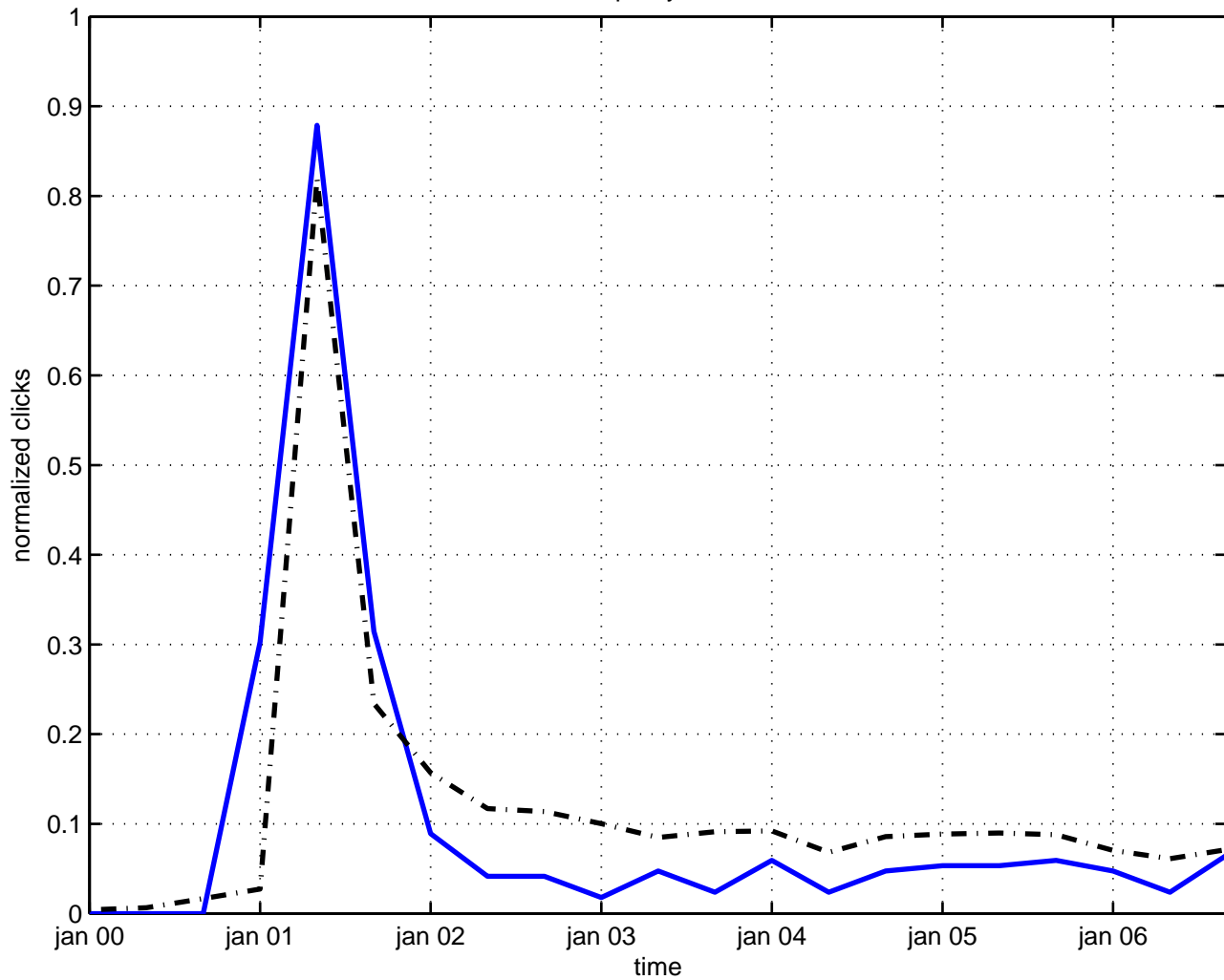
multiplicity fusion
