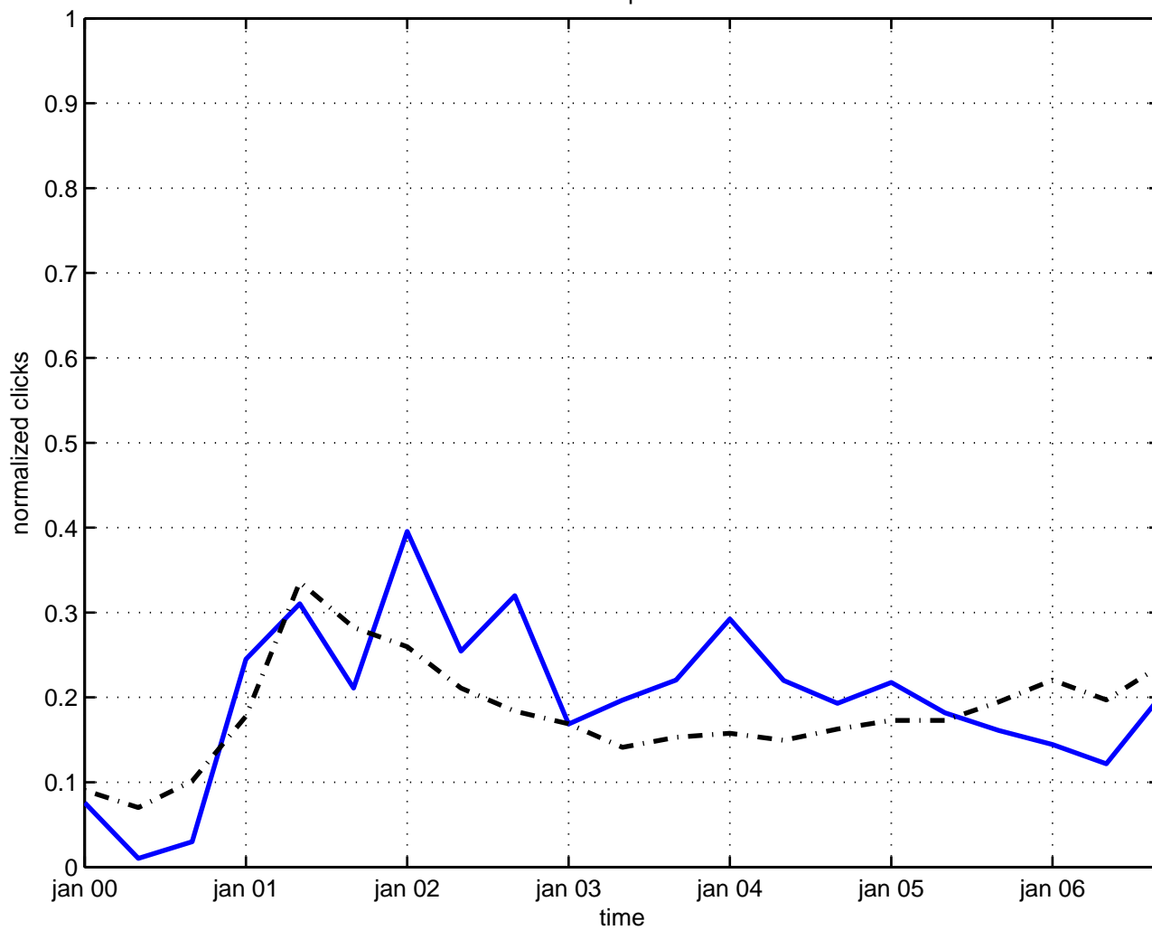
multiplet
