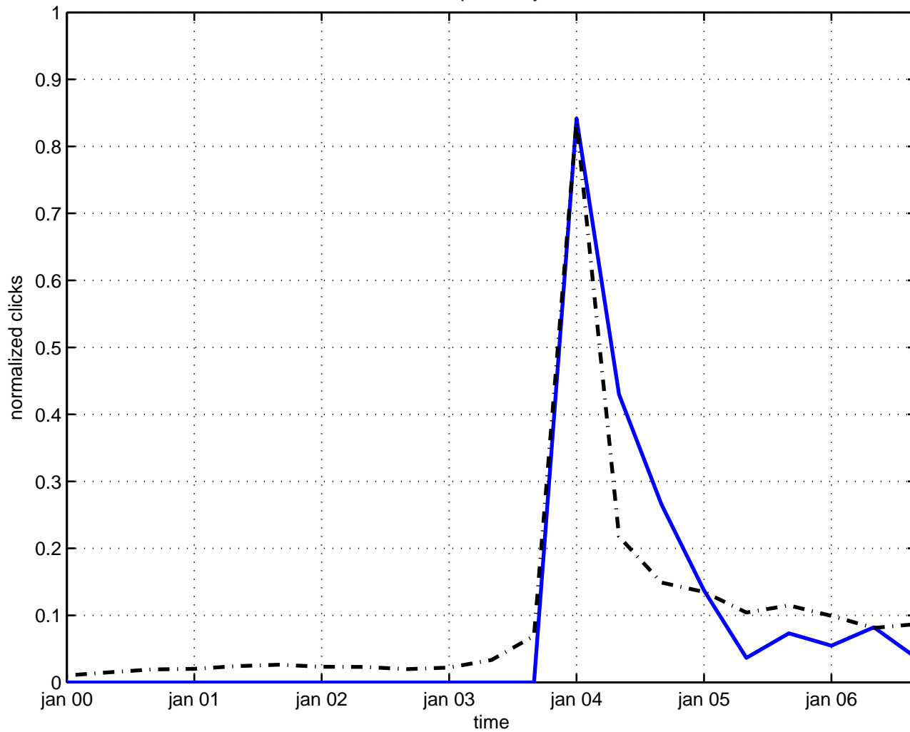
multiplet tachyon
