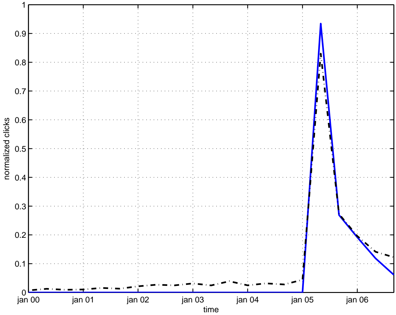
multiplet sparticle
