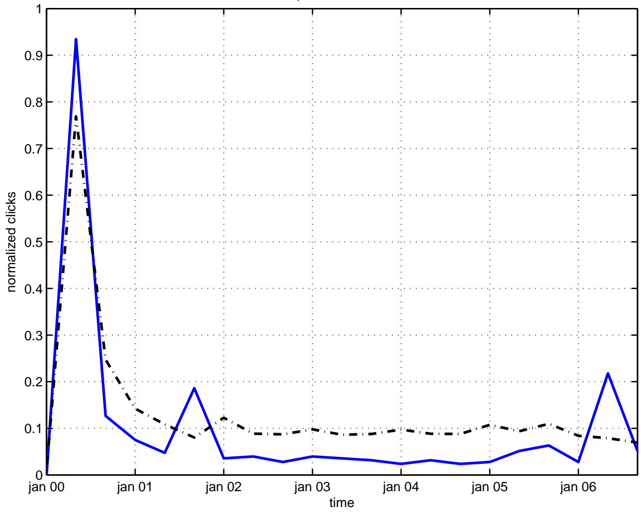
multiplet mass difference
