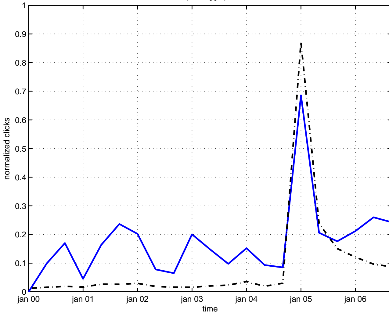
multiplet higgs particle
