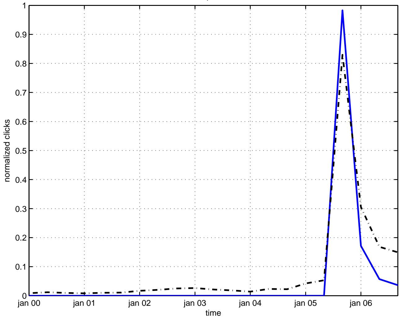
mu-problem
