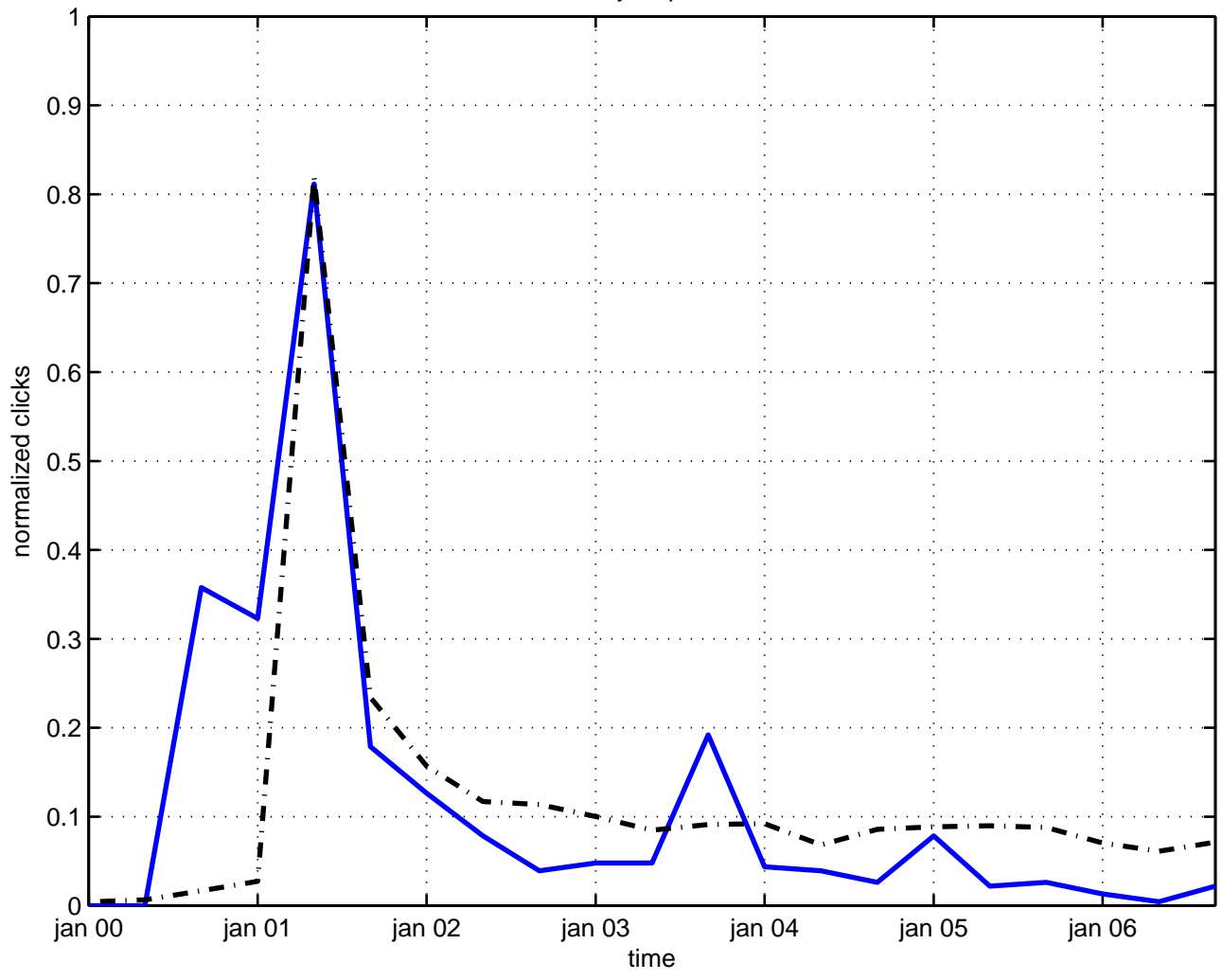
moyal space
