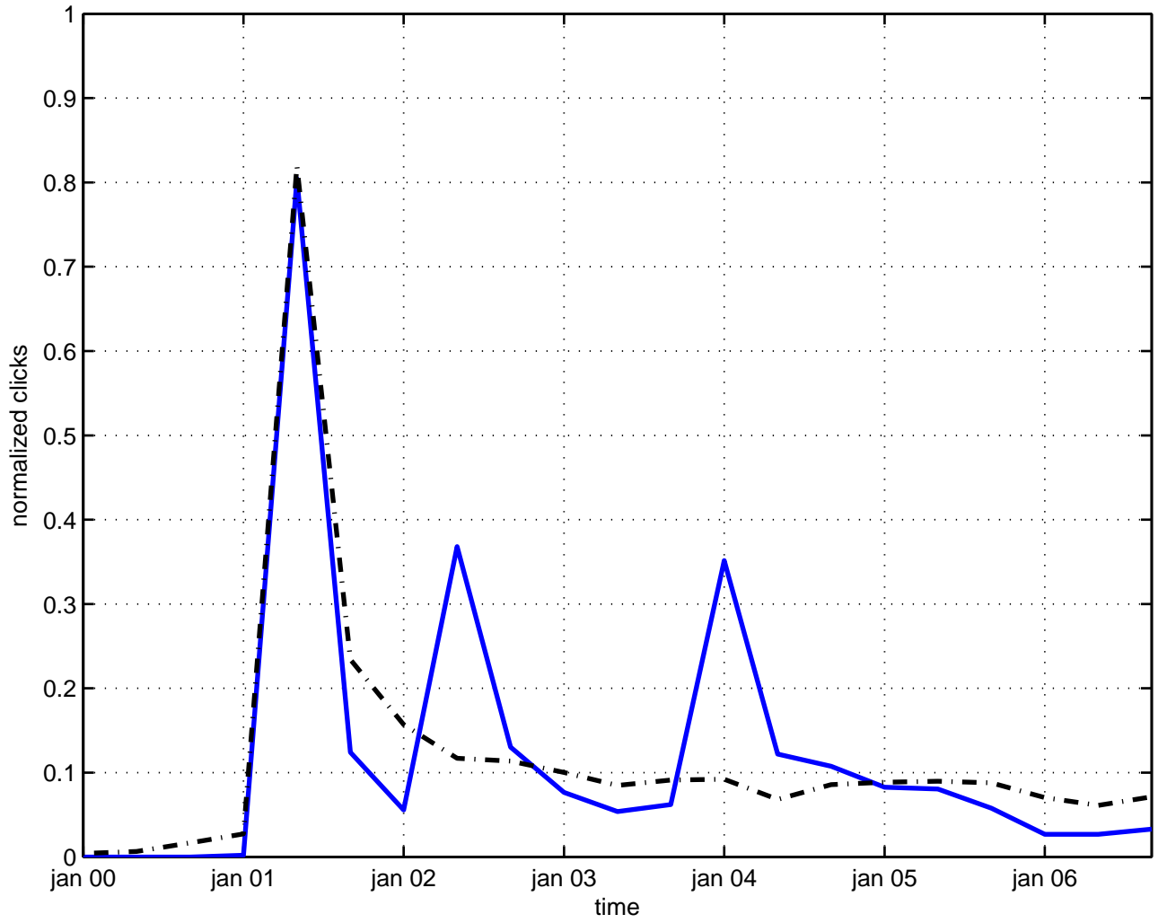
moyal quantization
