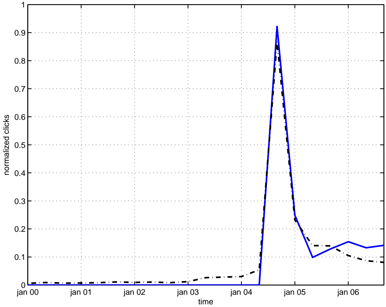
monopole perturbation
