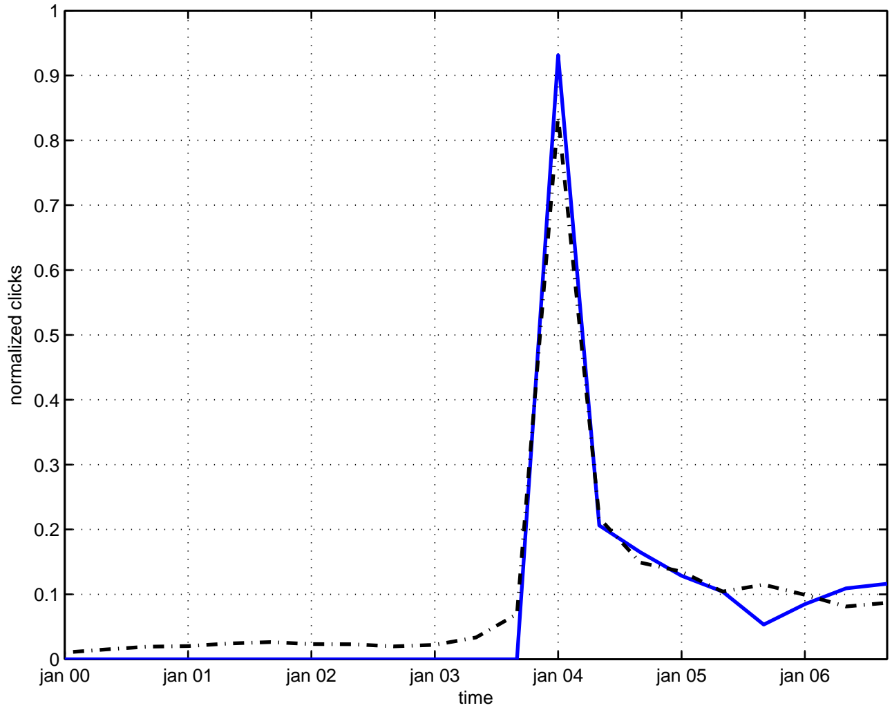
monopole kink
