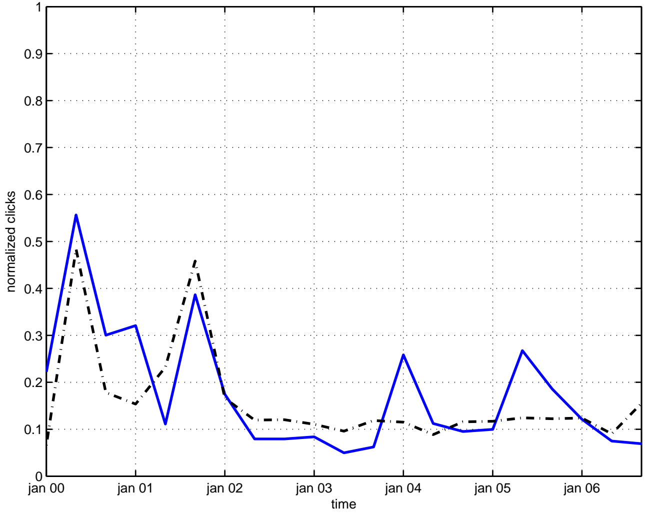
monopole kaluza-klein model
