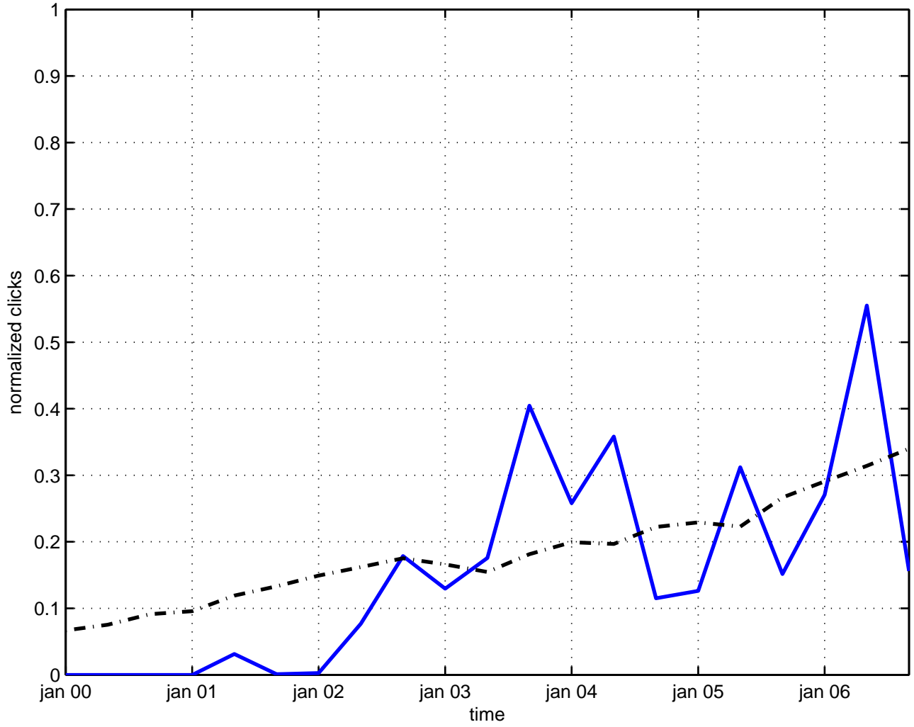
monopole field theory
