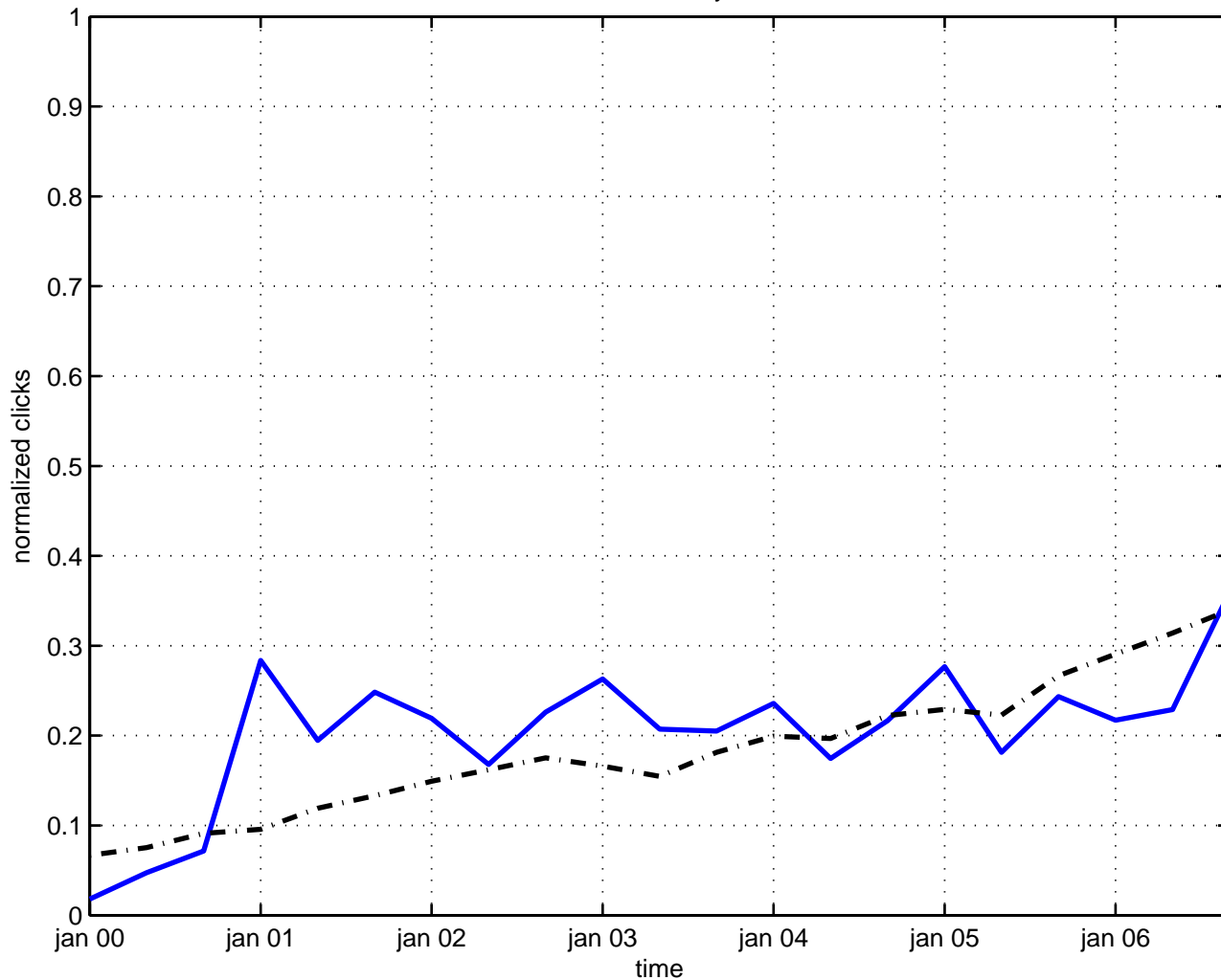
monodromy
