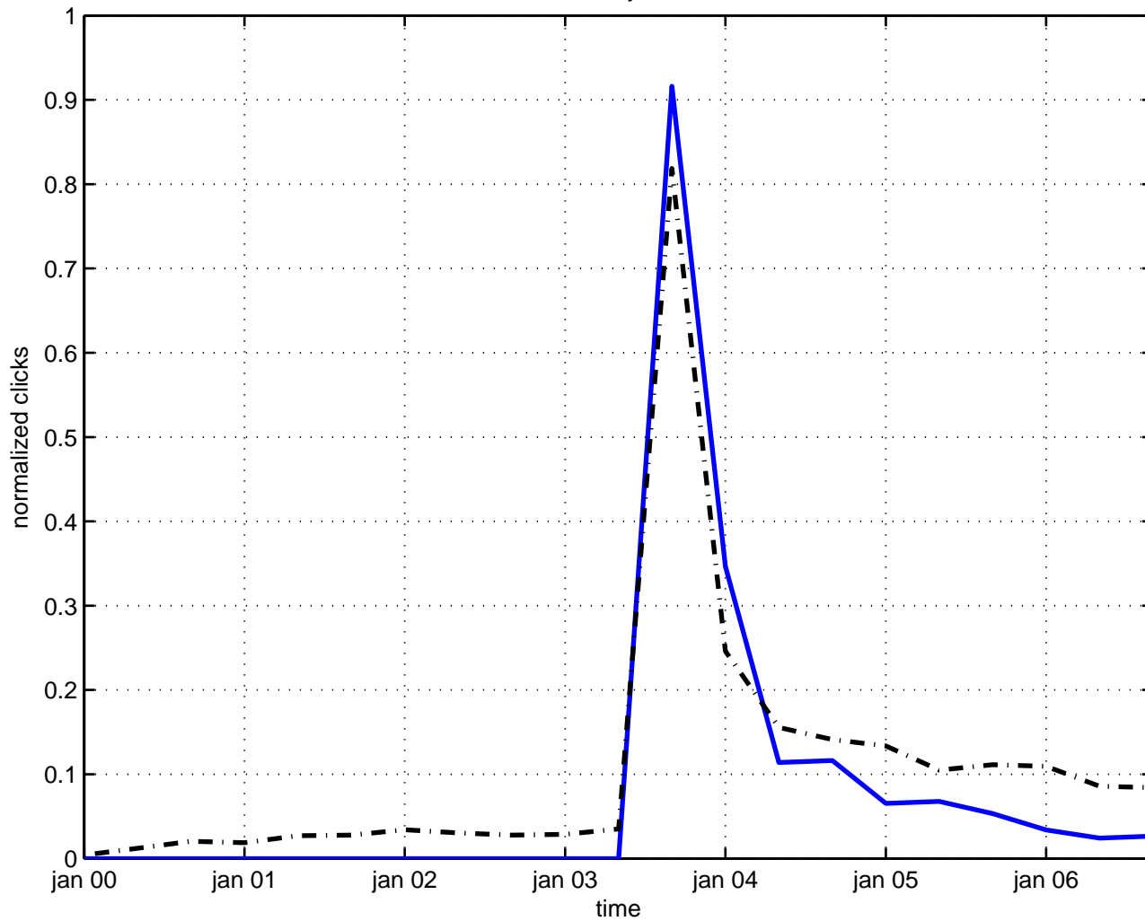
monodromy horizon
