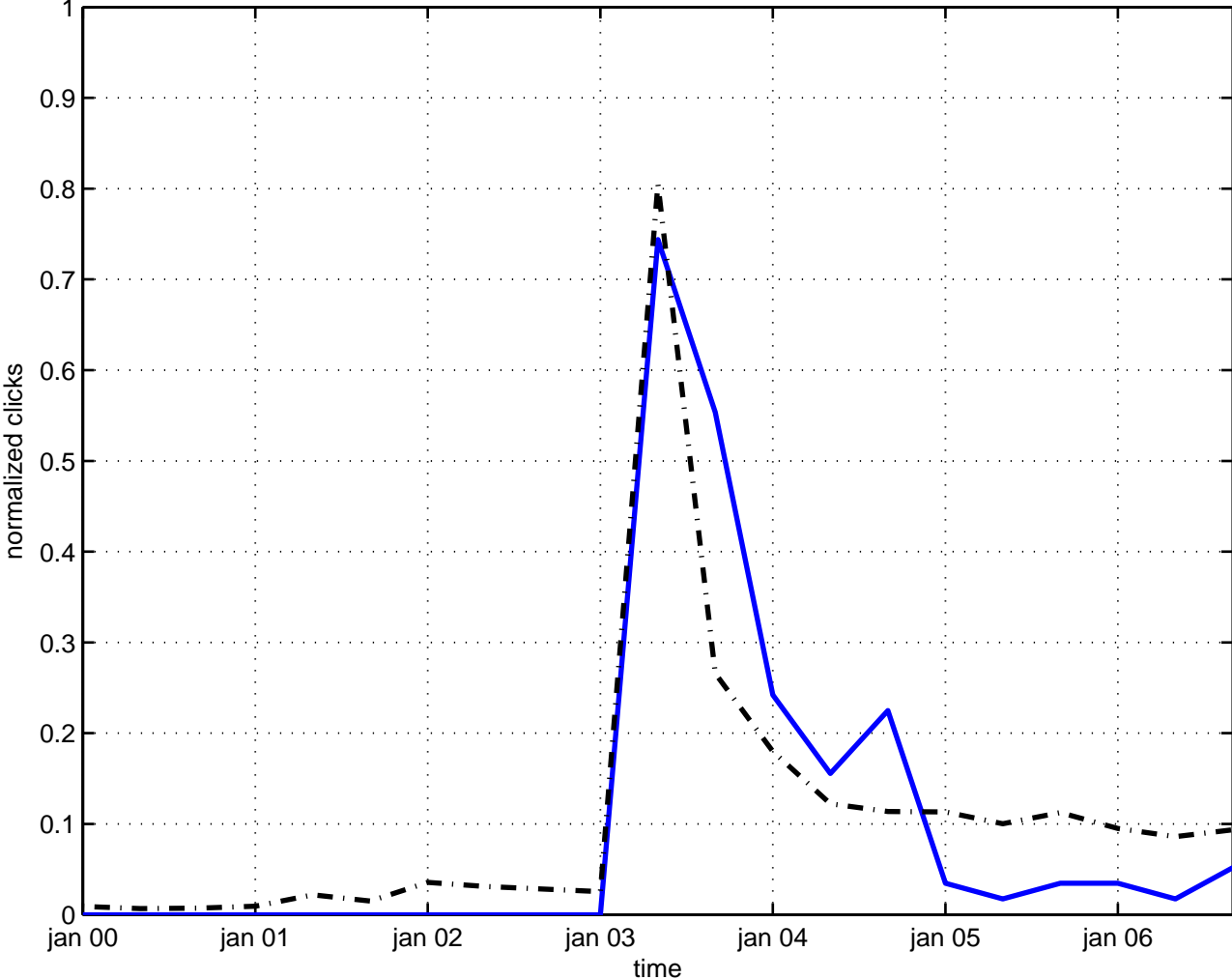
momentum transfer
