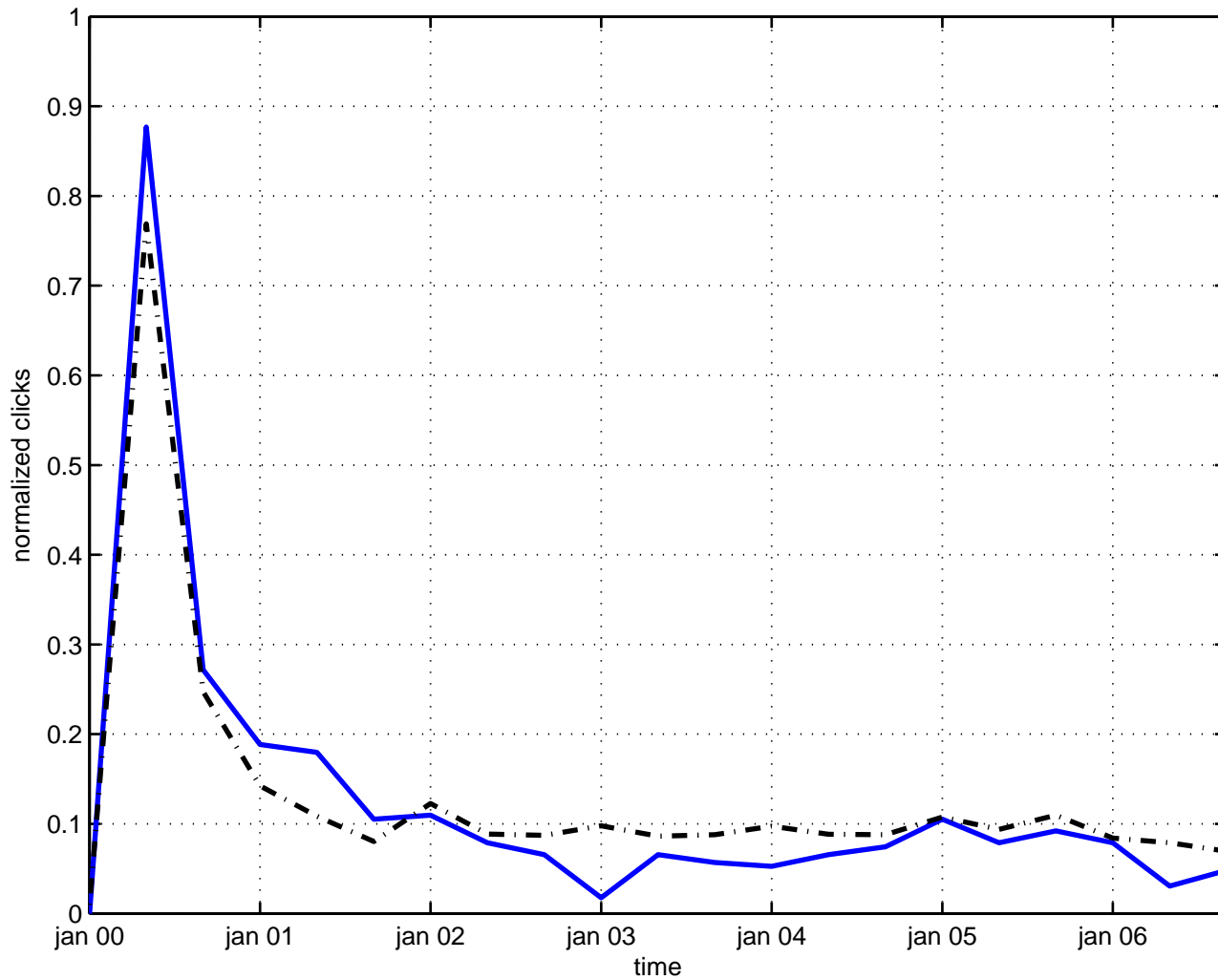
momentum soliton
