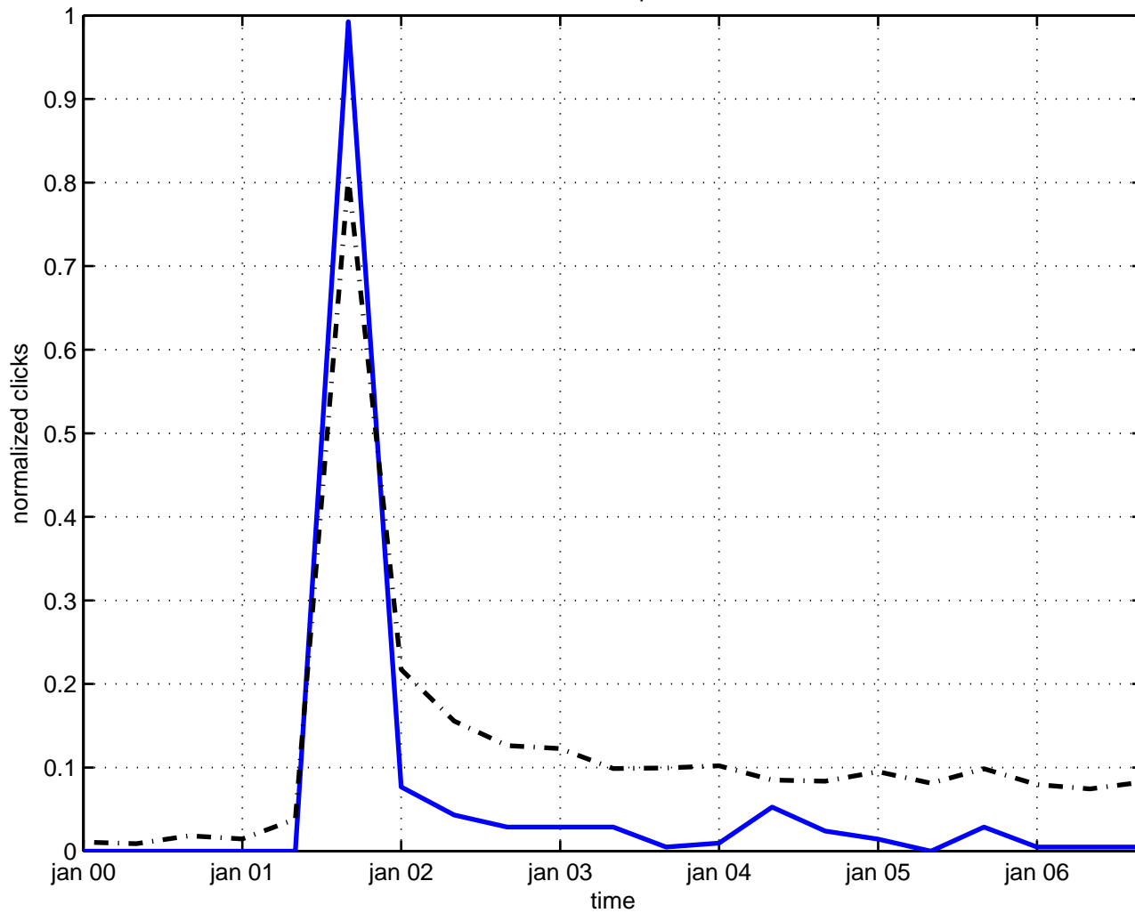
momentum photon
