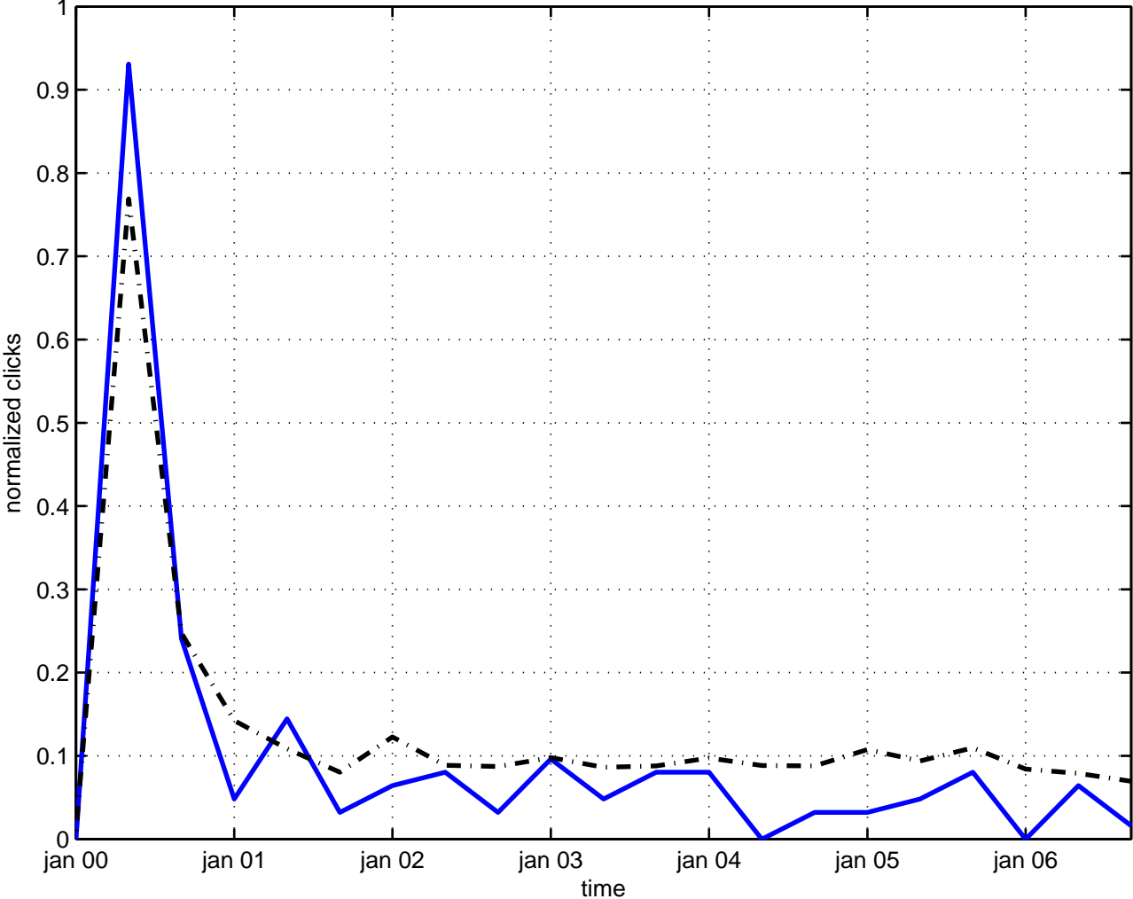
moduli string model
