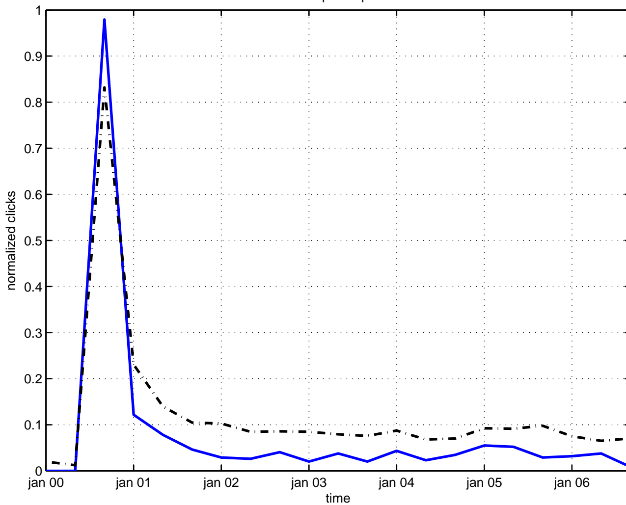
moduli space operator
