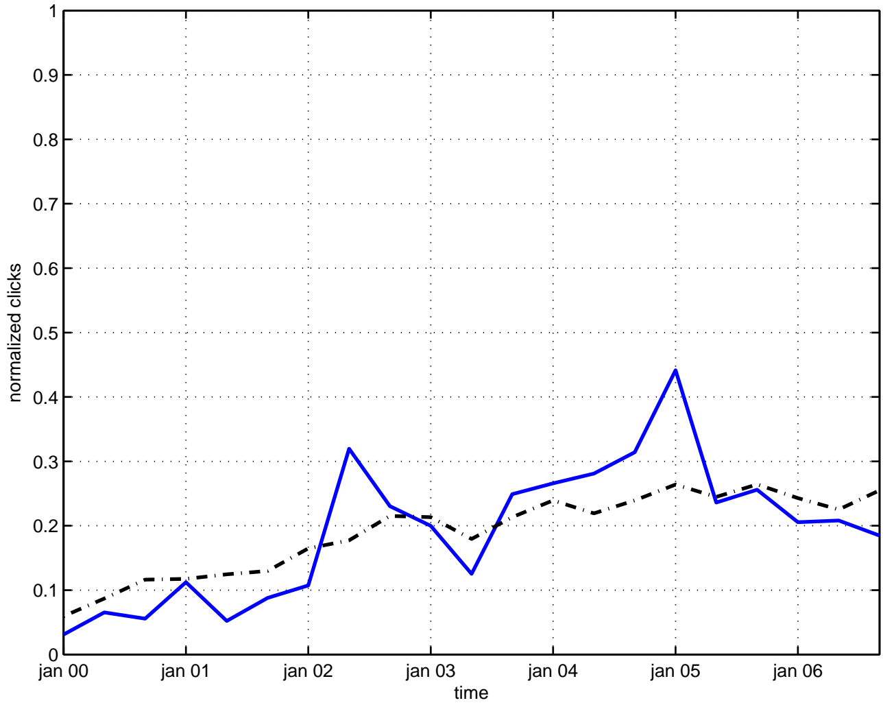
modular transformation
